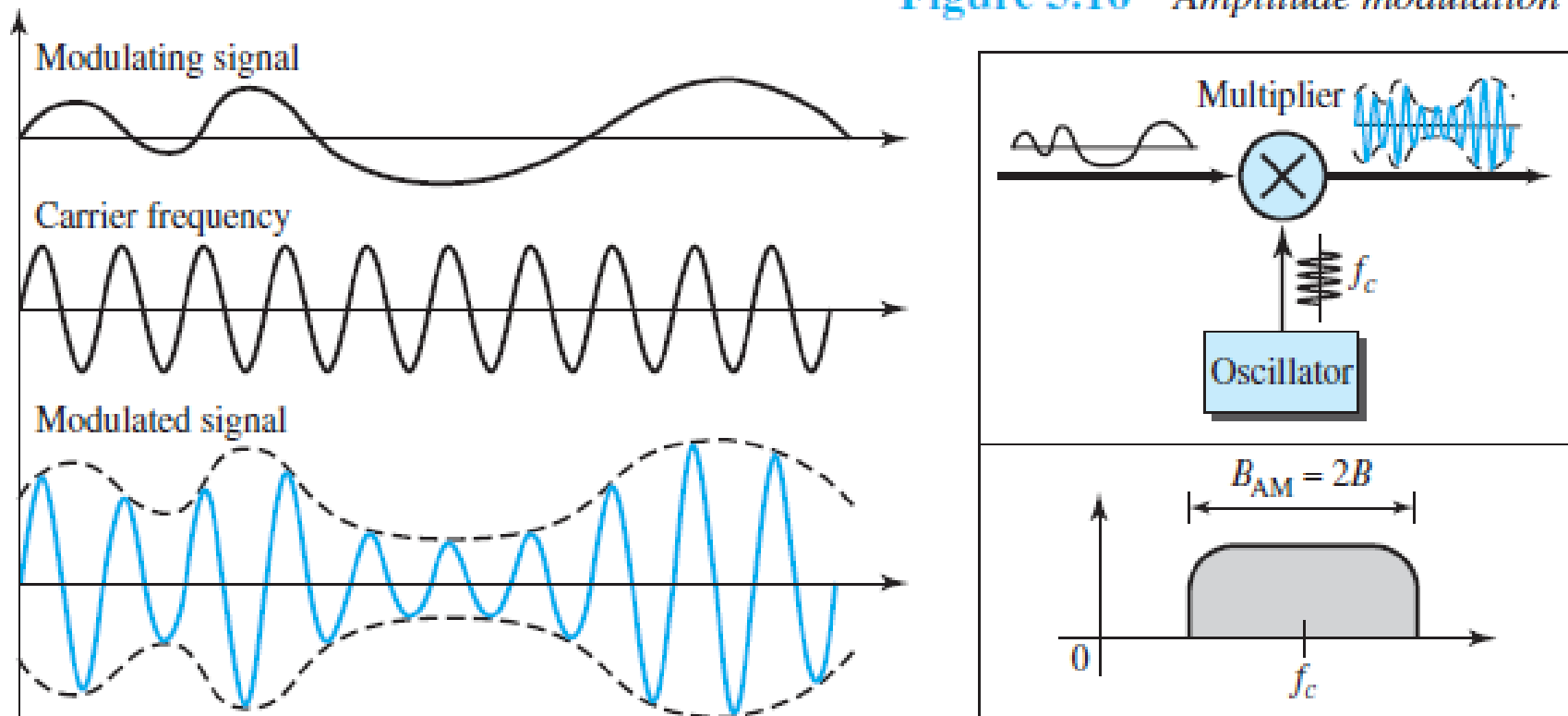
Figure 5.16 Amplitude modulation
