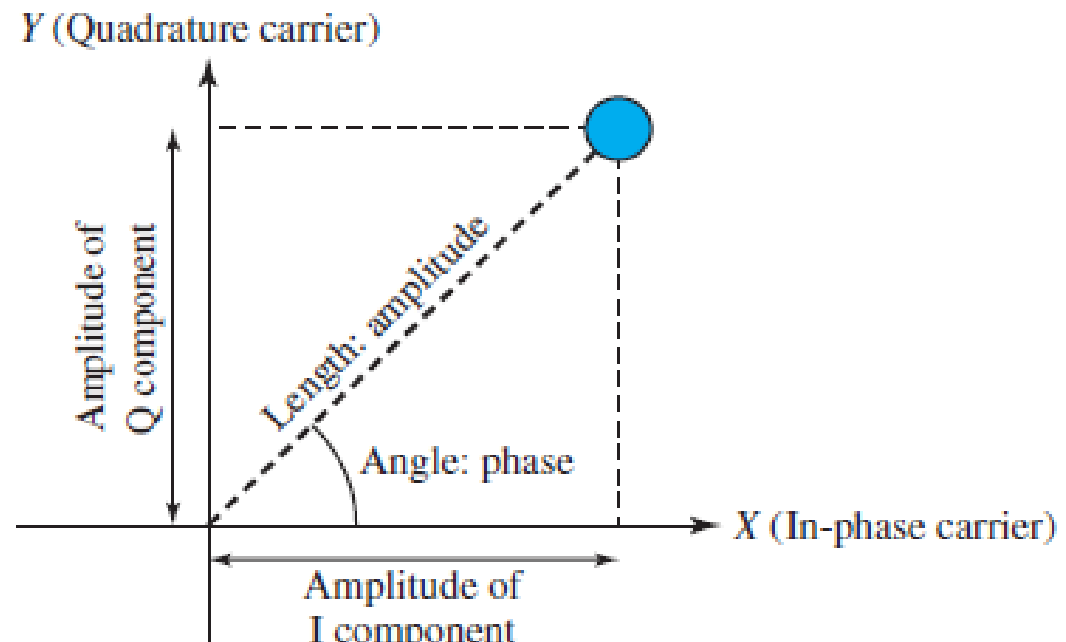
Figure 5.12 Concept of a constellation diagram
