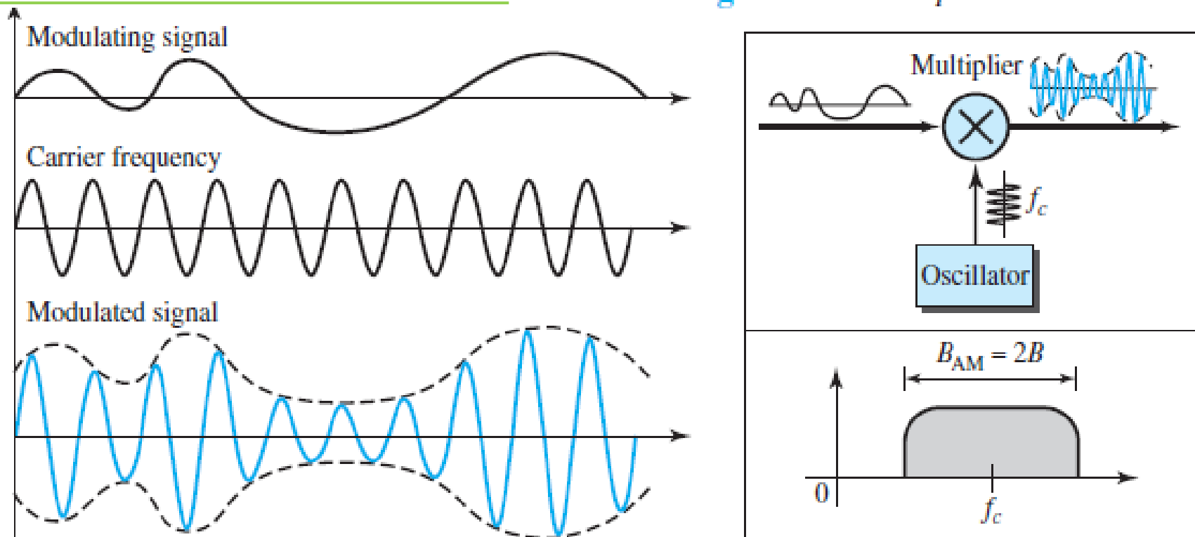
Figure 5.16 Amplitude modulation
