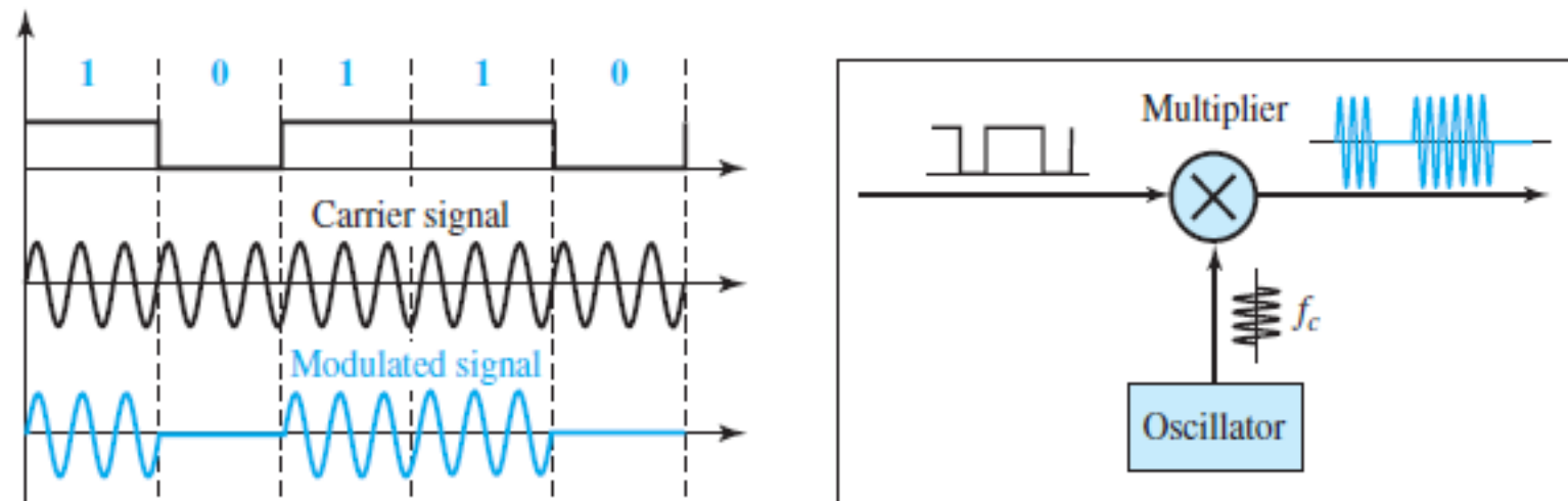
Figure 5.4 Implementation of binary ASK
