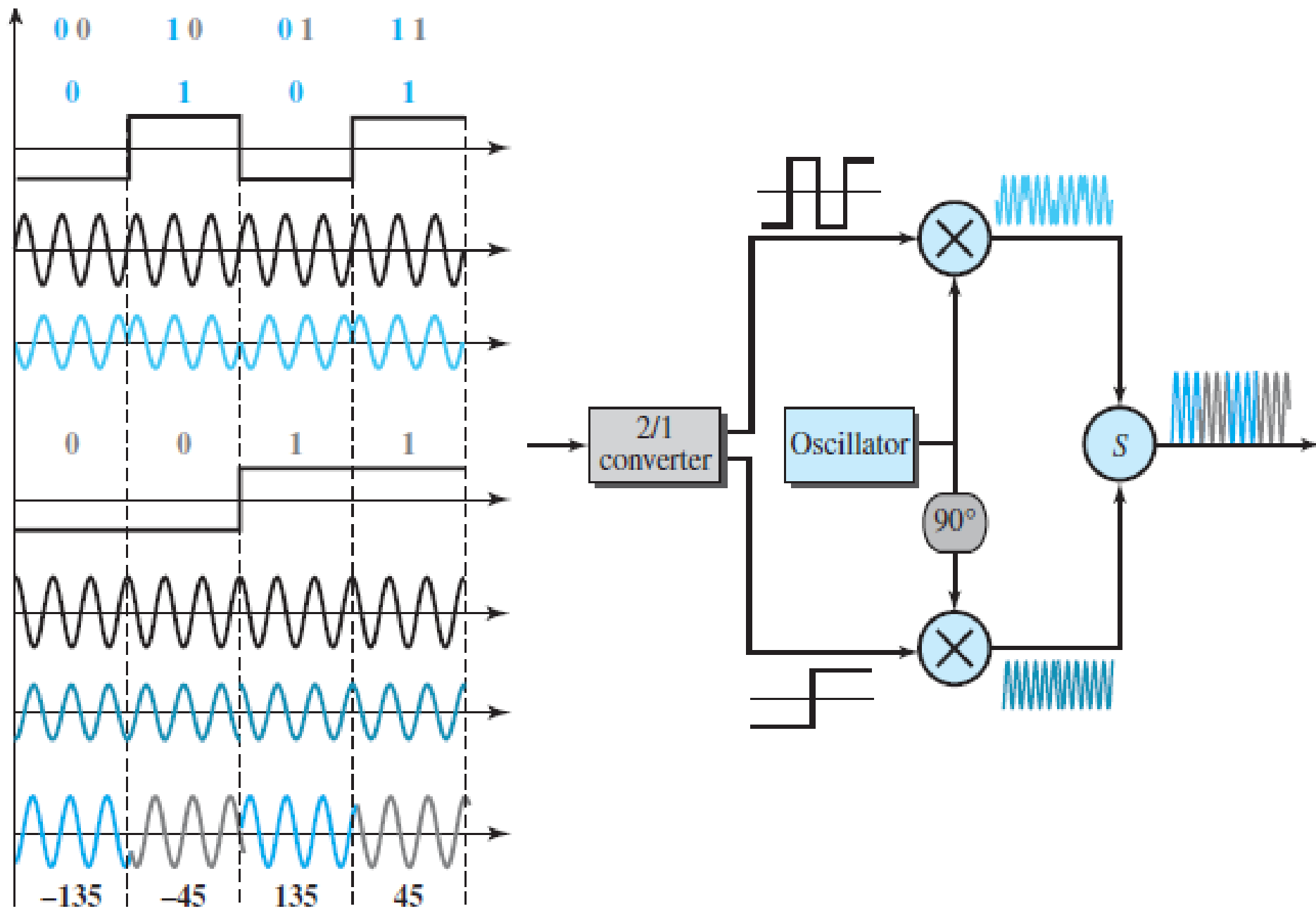
Figure 5.11 QPSK and its implementation
