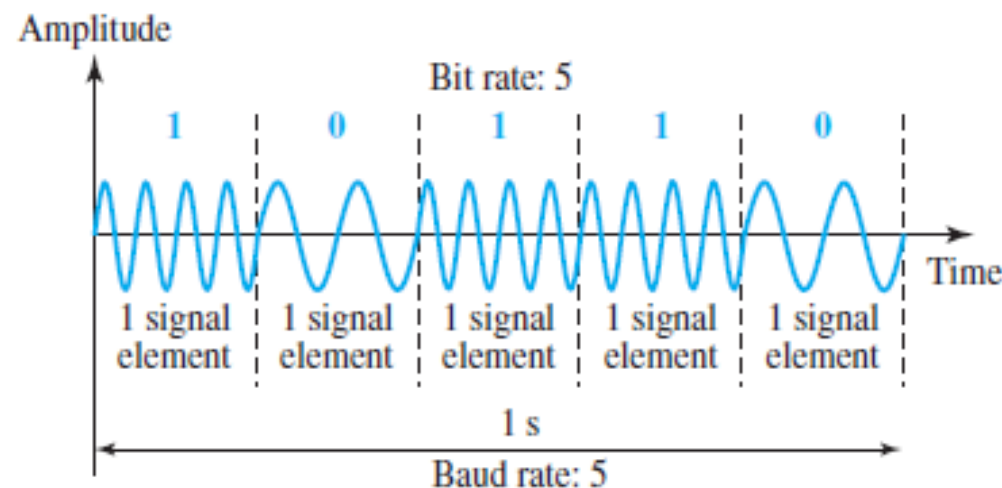
Figure 5.6 Binary frequency shift keying
