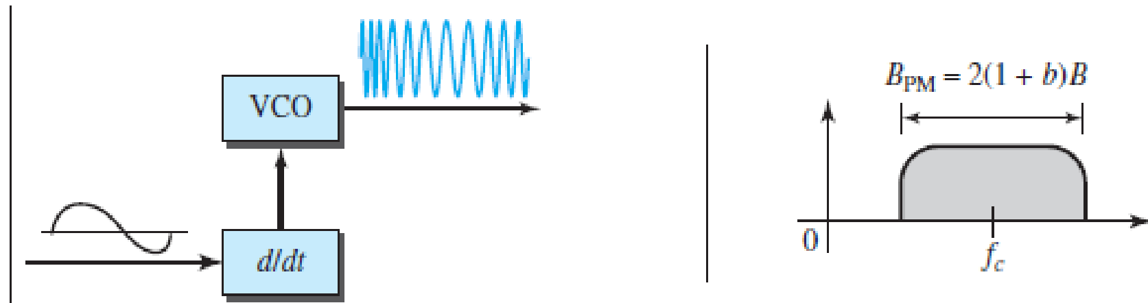
Figure 5.20 Phase modulation
