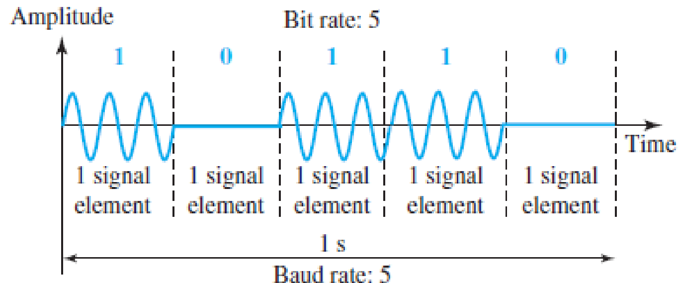
Figure 5.3 Binary amplitude shift keying
