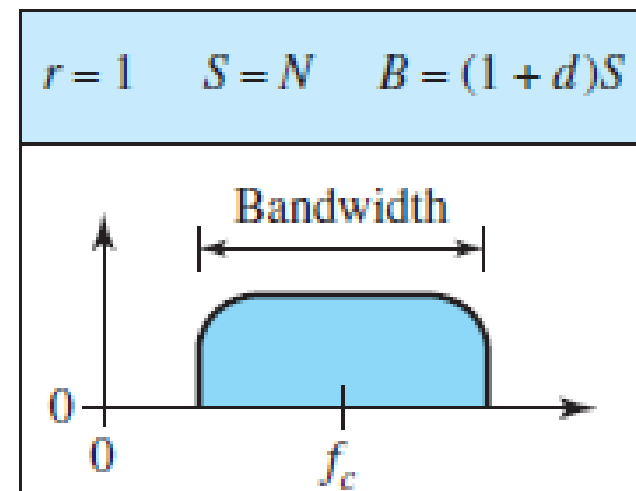
Figure 5.3 Binary amplitude shift keying
